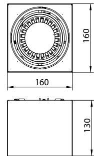
Technical drawing
