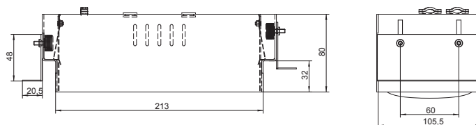
Technical drawing
