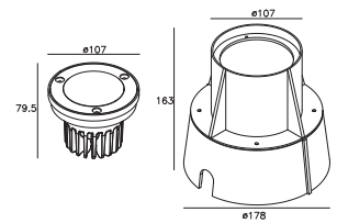
Technical drawing
