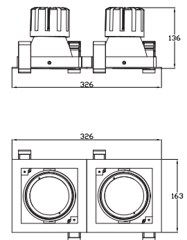
Technical drawing
