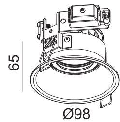
Technical drawing
