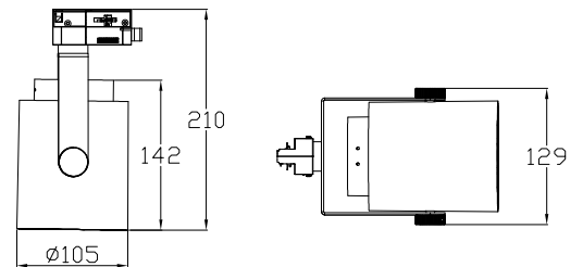
Technical drawing
