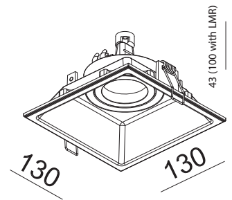
Technical drawing
