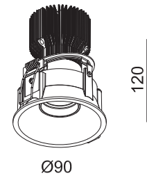
Technical drawing
