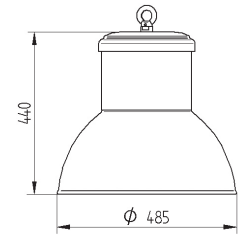
Technical drawing
