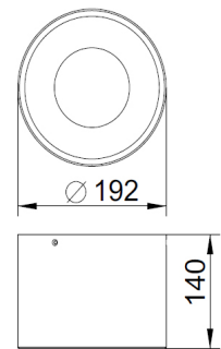
Technical drawing
