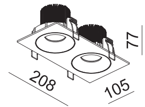
Technical drawing
