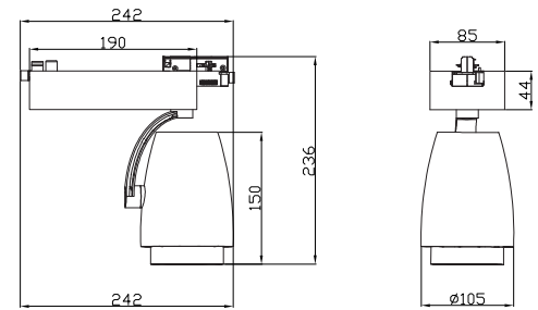
Technical drawing
