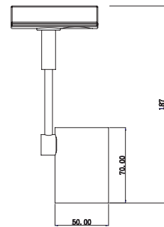
Technical drawing
