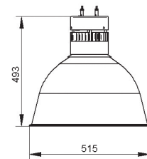
Technical drawing
