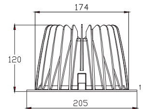
Technical drawing
