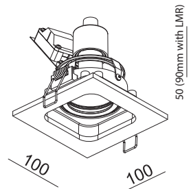
Technical drawing
