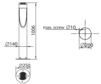
Technical drawing
