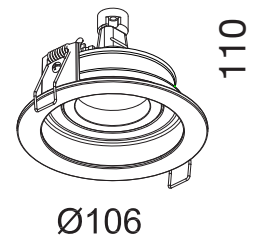
Technical drawing
