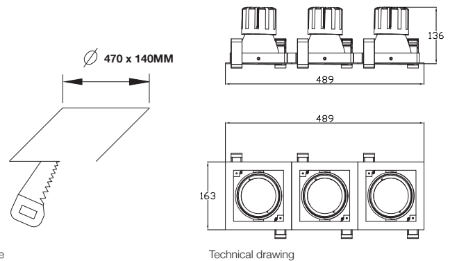
Technical drawing
