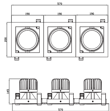
Technical drawing
