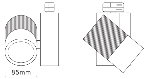
Technical drawing
