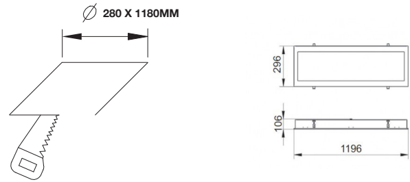
Technical drawing
