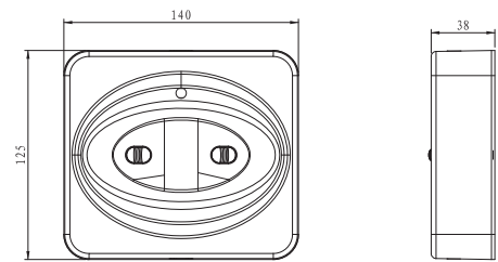
Technical drawing
