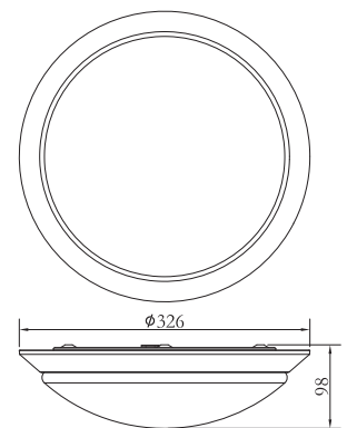
Technical drawing
