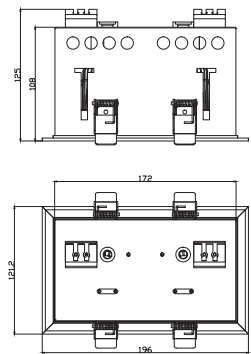
Technical drawing
