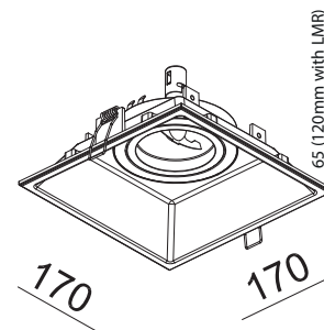
Technical drawing
