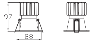
Technical drawing
