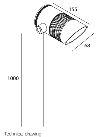
Technical drawing
