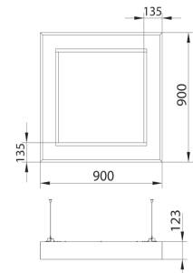
Technical drawing
