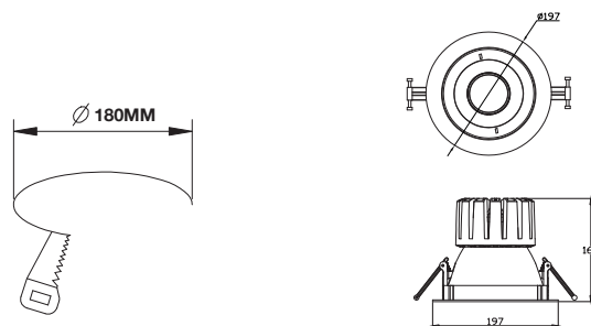
Technical drawing
