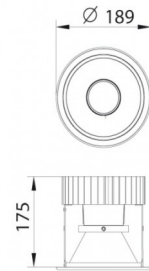
Technical drawing
