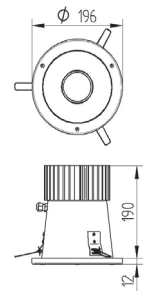
Technical drawing
