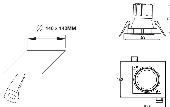
Technical drawing
