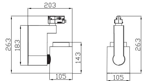
Technical drawing
