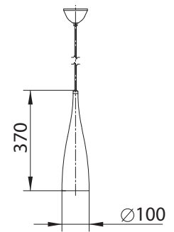
Technical drawing
