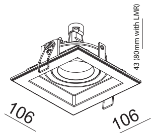
Technical drawing
