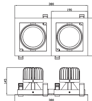
Technical drawing
