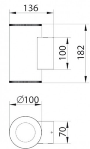
Technical drawing
