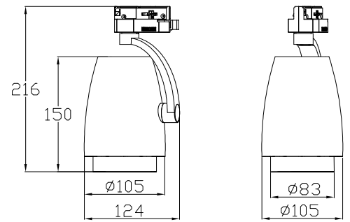
Technical drawing
