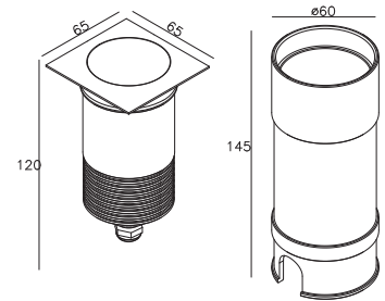
Technical drawing
