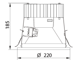
Technical drawing
