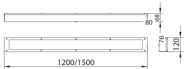
Technical drawing
