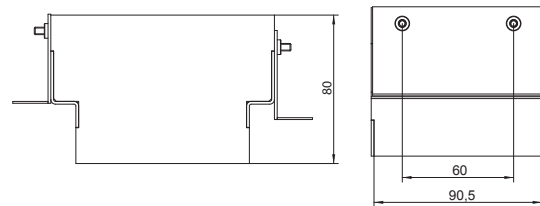
Technical drawing (Mounting plasterkit)
