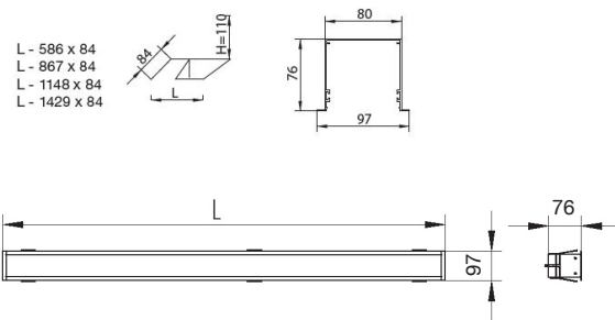
Technical drawing
