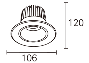
Technical drawing
