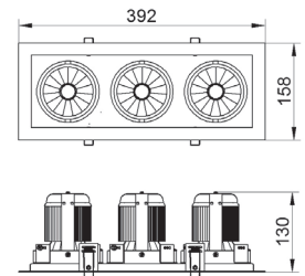
Technical drawing
