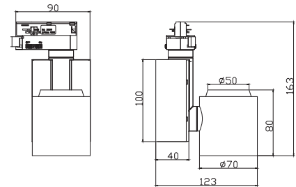
Technical drawing
