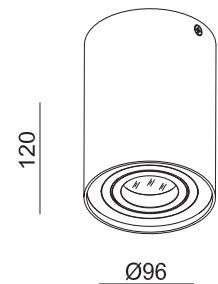
Technical drawing
