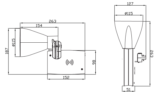
Technical drawing
