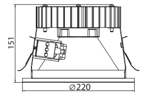
Technical drawing
