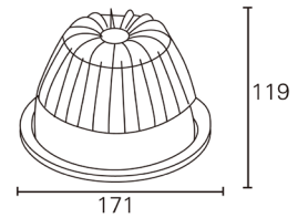
Technical drawing
