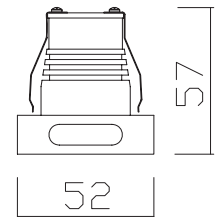
Technical drawing (square)
