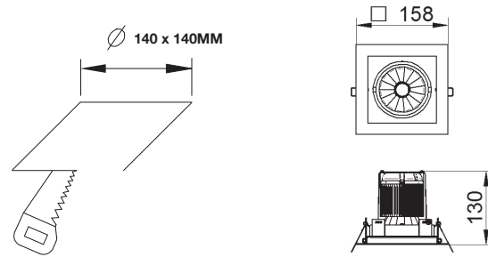
Technical drawing
