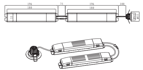
Technical drawing
