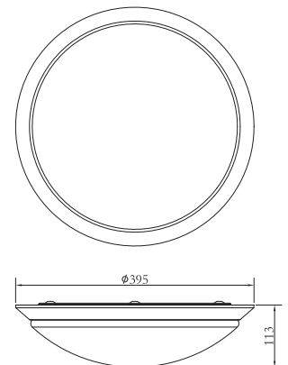
Technical drawing
