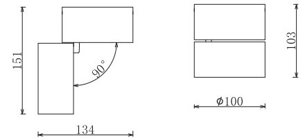
Technical drawing
