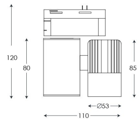
Technical drawing
