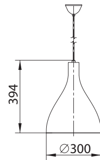
Technical drawing
