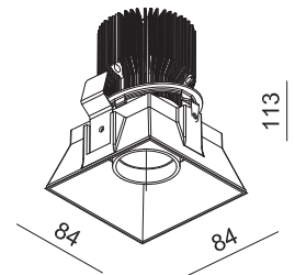
Technical drawing
