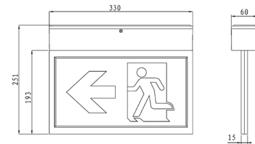
Technical drawing
