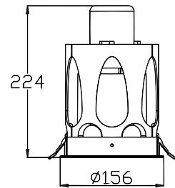
Technical drawing
