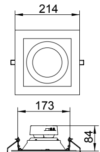
Technical drawing
