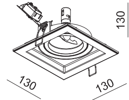
Technical drawing
