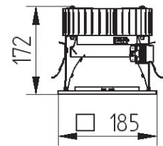
Technical drawing
