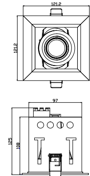
Technical drawing
