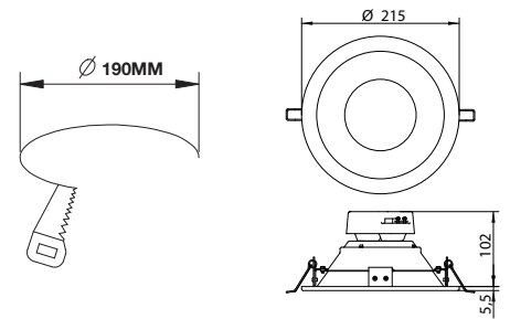
Hole size
